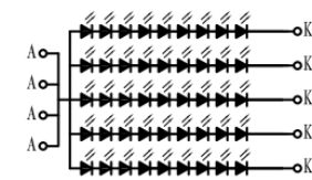
Backlight LED Circuit
